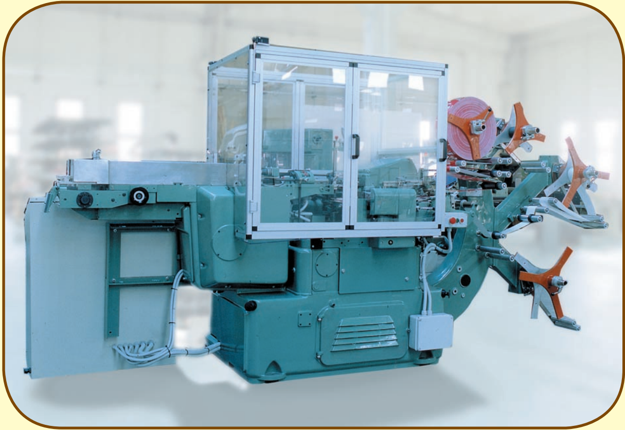
Rebuilt ACMA 711 Wrapper
